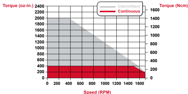
DPP703-410 & DPP703M-290
